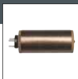
Item No. 3071 Grajač 2x2000 W, 230 V
